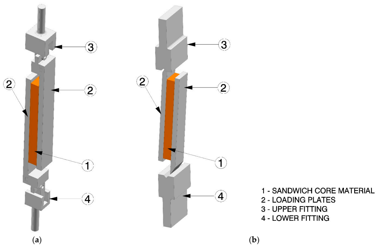
Figure 1. Schematic representation of the specimen designed according to the ASTM C273 standards for: (a) specimen loaded in the tensile direction; and (b) specimen loaded in the compressive direction.
