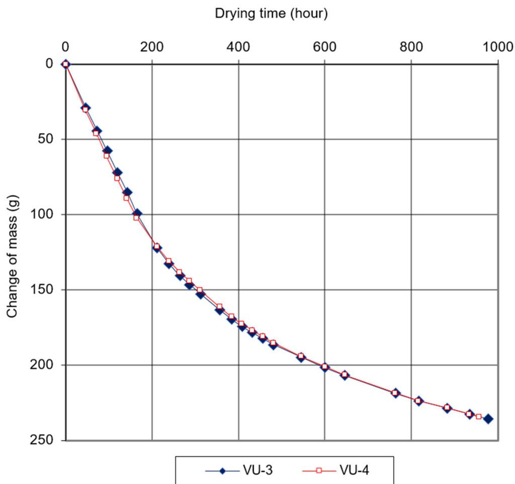
Figure 5. Mass loss of samples (twins) during drying in the laboratory.
