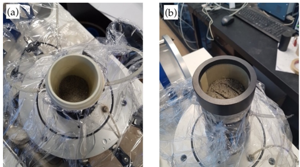
Figure 6. Sample preparation using undercompaction method: (a) lower layers of compaction, and (b) upper layers of compaction, according to [24].
