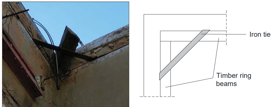
Figure 6. Connection of timber ring beams at a corner via iron ties.
