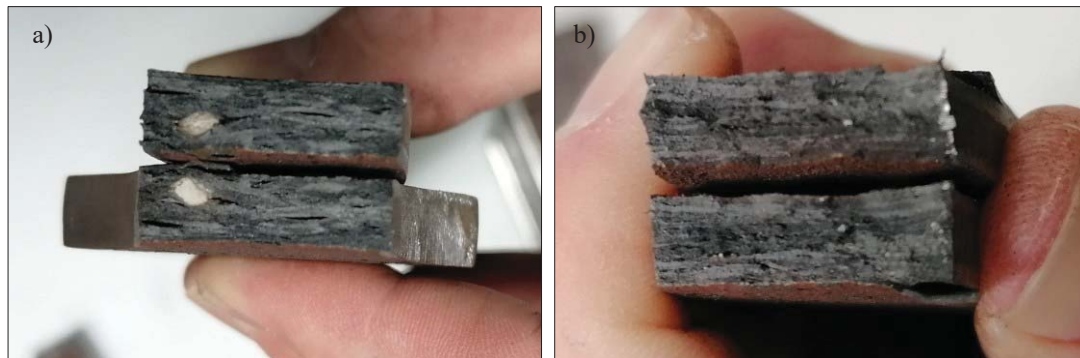
Figure 14. Fracture surfaces: a) Specimen 2; b) Specimen 3.
