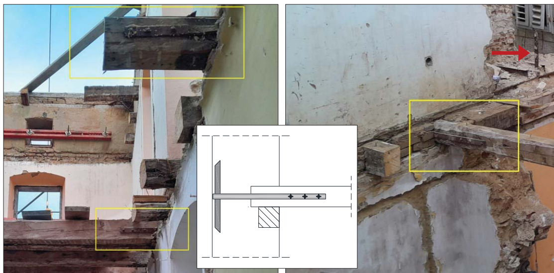
Figure 7. Horizontal wall-to-floor ties.
