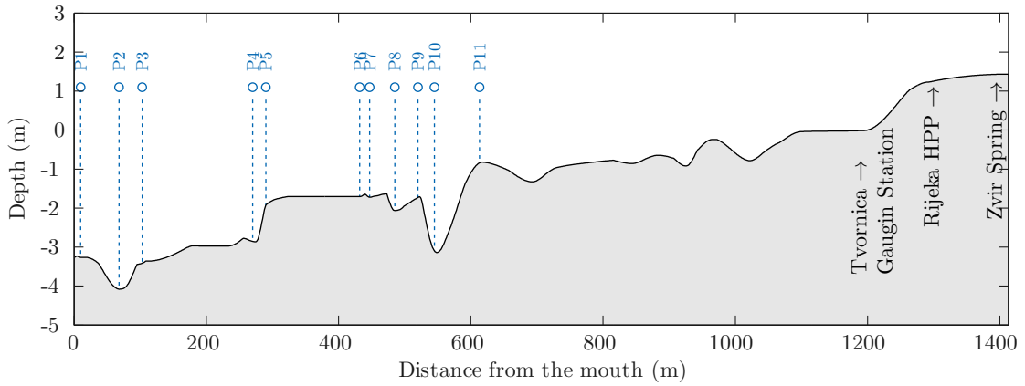
Figure 6.12: Longitudinal section of the Rječina River estuary with bed elevations and locations of sampling points.
