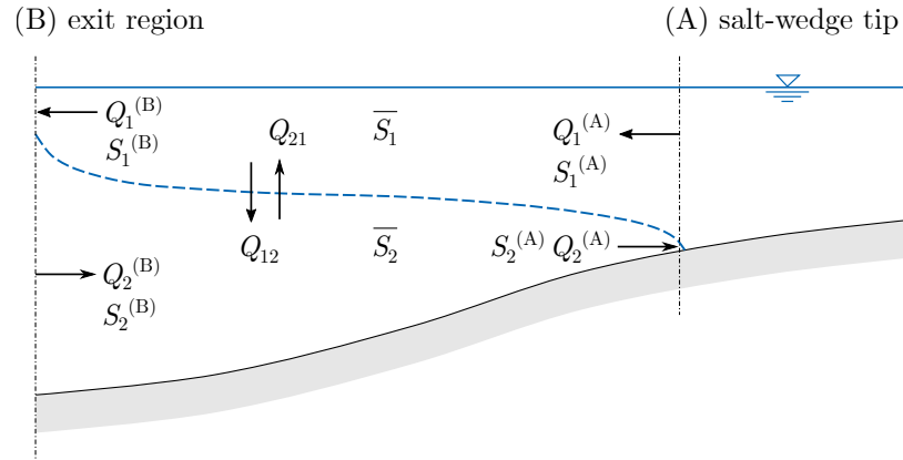
Figure 6.10: Scheme of a two-layer box model for estimating the vertical mixing in salt-wedge estuaries.
