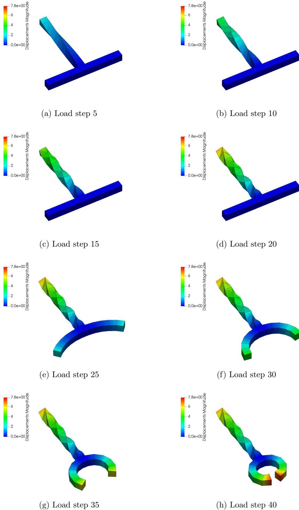
Figure 5.8: Deformed configuration of the T-shape structure for different load steps obtained using 21 \times 1 \times 1 Hex8NL for M_1 = 1200 Nmm, M_2 = 2250 Nmm
