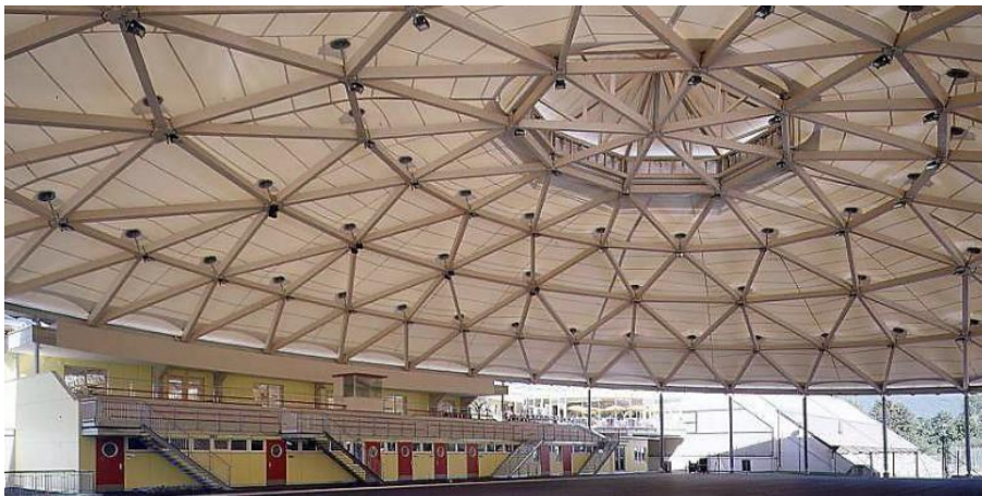
Slika 35: Sportski centar Telfs, Austrija (Indermühle Bauingenieure 1999)
