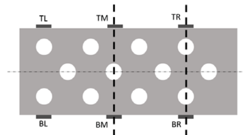
Fig. 4. Position of the strain gauges on B3 sample in pure bending zone.
