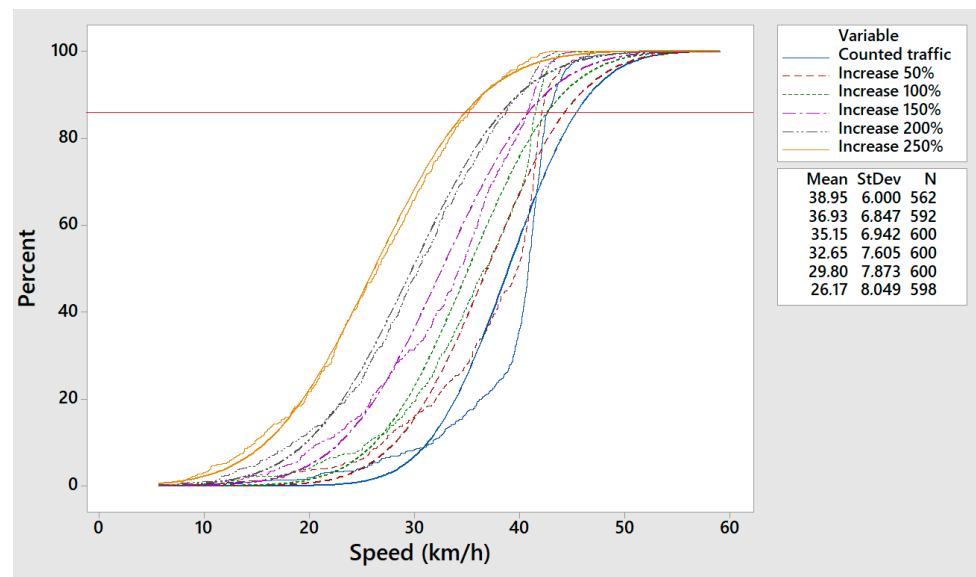
Figure 7. Cumulative speed diagram for a reconstructed pedestrian crosswalk (normalized).
