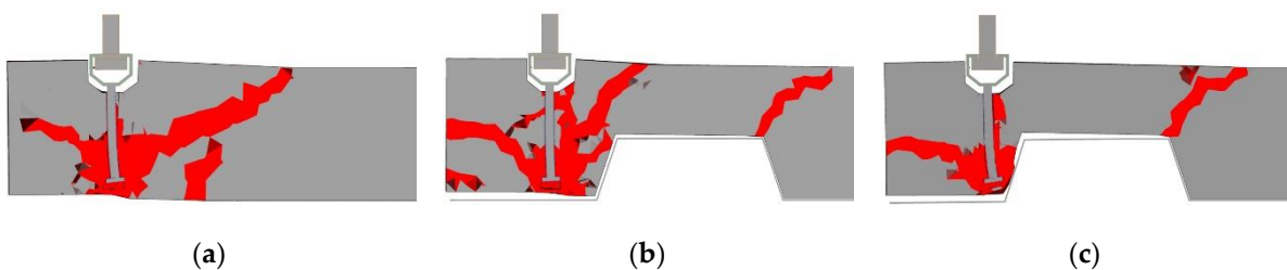
Figure 5.17 Post-peak breakout patterns (section through the anchor for h_{ef} = 120 \text{ mm} ) for: (a) plain concrete slab; (b) composite slab - d_w = 45 \text{ mm} ; (c) composite slab - d_w = 15 \text{ mm}
