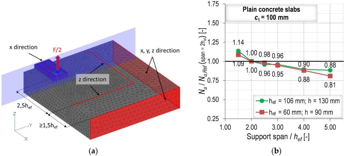
Figure 4.7 (a) FE model used in the numerical parametric study; (b) Influence of support span
