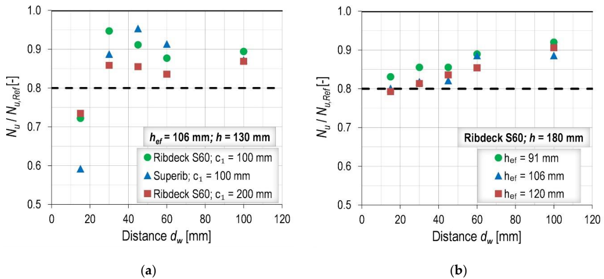
Figure 5.16 Numerical results of Series 1 for: (a) the embedment depth h_{ef} = 106 \text{ mm} ; (b) the overall member thickness h = 180 \text{ mm}
