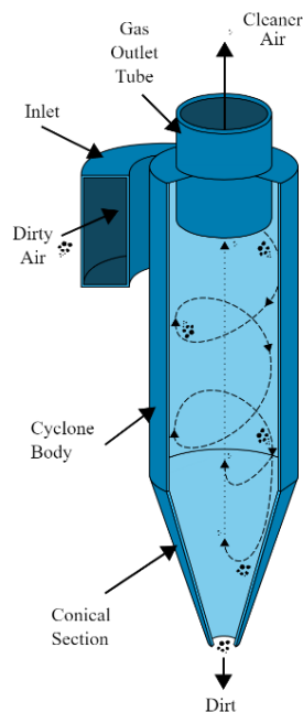
Slika 30: Ciklonski separator [ https://energyeducation.ca/encyclopedia/Cyclone_separator ]
