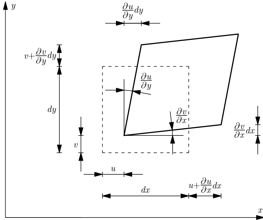
Figure 2.2: Differential 2D element after displacement and deformation
