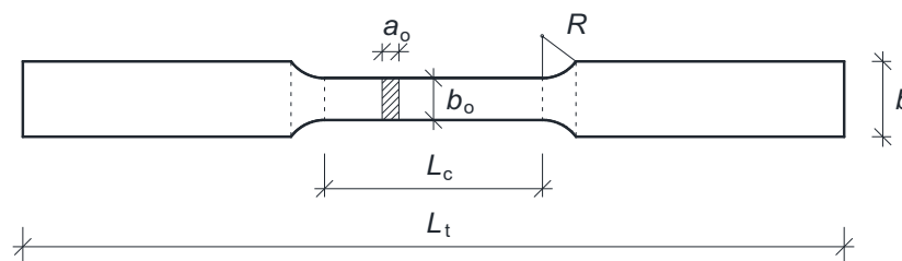
Figure 11. Specimen details.
