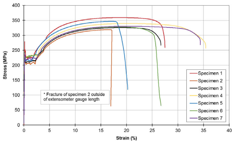
Figure 13. Stress-strain diagram of iron ties.
