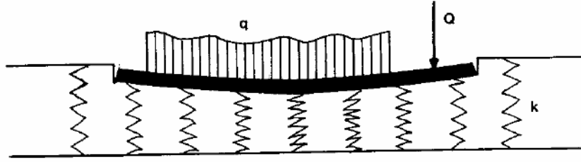
Figure 1: Winkler's model [12]
